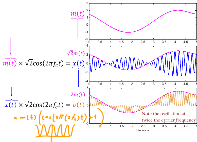
Figure 20: DSB-SC modem: signals in time domain
