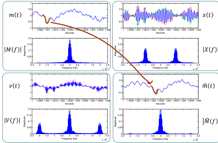
Figure 19: DSB-SC modem: signals and their spectra (zooming in)
